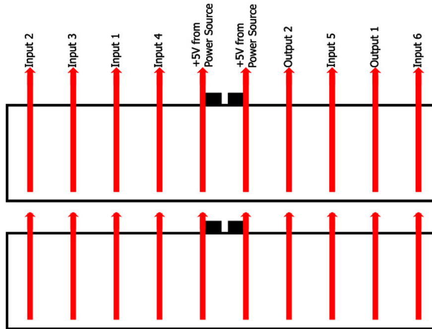
Rear (Wire-Side) View of IDC Connector
