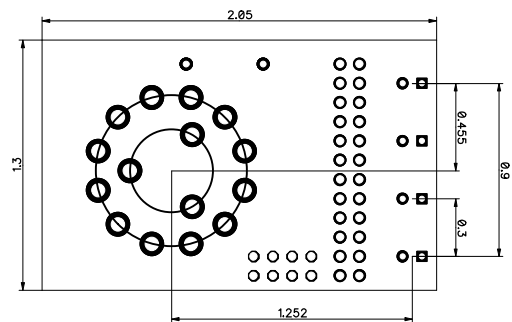
Switch bushing: M9x0.75 (3/8"-32NEF)
